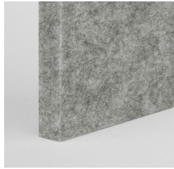
ATOM
