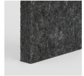
GALAXY
